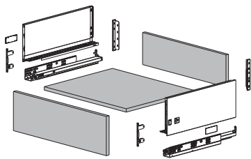
Product Breakdown Drawing
